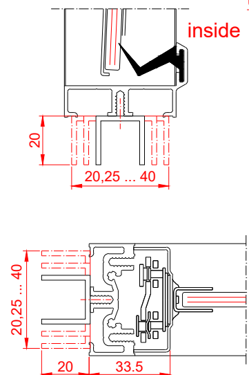
Detail glazingprofile
